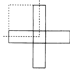
Figure 1 The procedure of BM 13901 N° 23.
