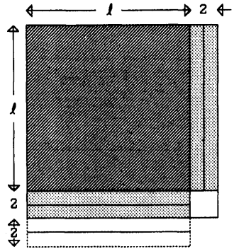
Figure 2 The procedure described in Geometrica 24.3.
